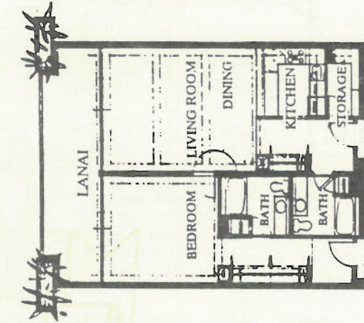
FLOOR PLAN - C
