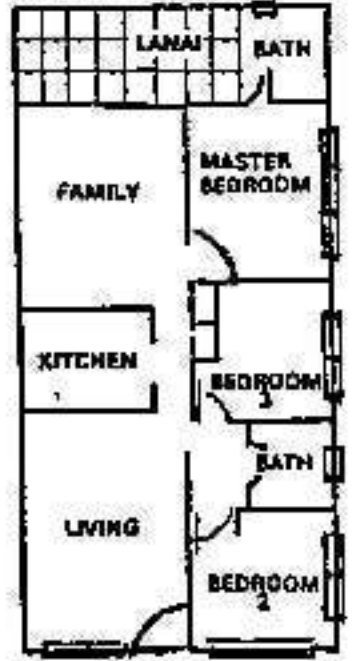
THREE BEDROOM ONE STORY 1594 S.F.
